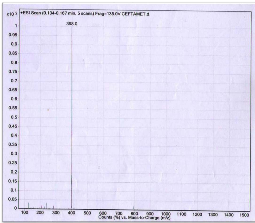
Figure 5: Mass Spectra of Cefetamet Sodium
