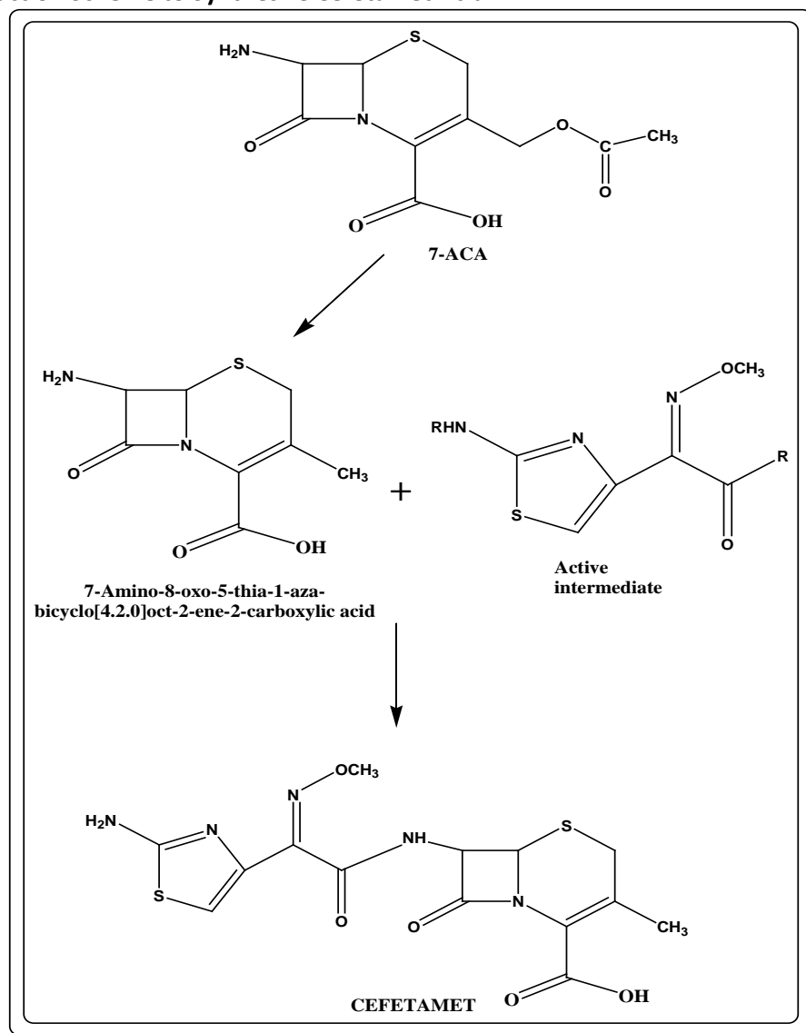
Figure 2: Scheme to Synthesize Cefetamet Acid
