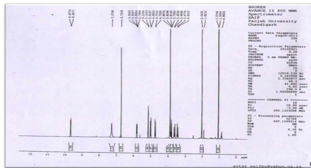
Figure 4: NMR Spectra of Cefetamet
