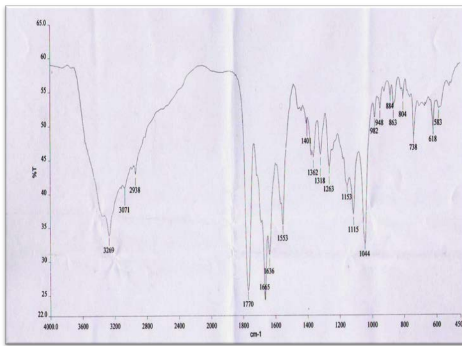
Figure 6: I.R. Spectra of Cefetamet
