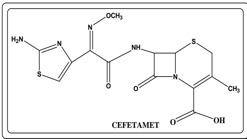
Figure 1: Structure of cefetamet
